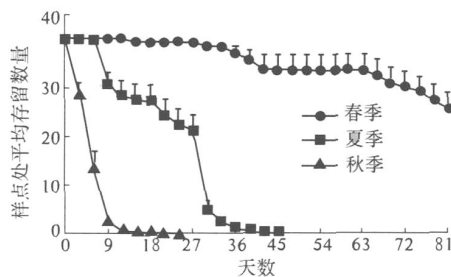
图1 不同季节山杏种子在释放点的存留动态 Fig.1 Survival dynamics of released seeds of Prunus armeniaca among different seasons
